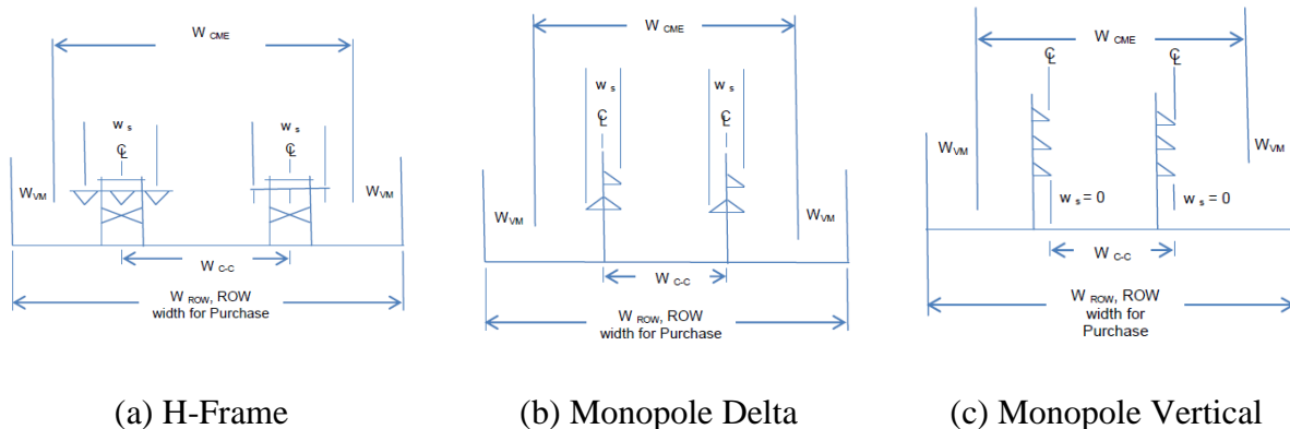
Figure 6.3.4.1-2 – Typical Double Structure ROW
